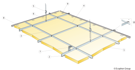
Installation diagram (M500) for Ecophon Master Eg
