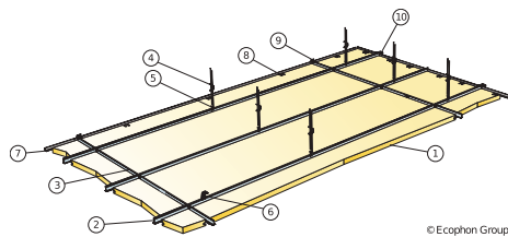
Installation diagram (M500) for Ecophon Master Eg
