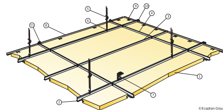
Installation diagram (M499) for Ecophon Master Eg
