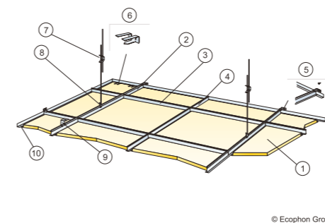
M204 Installation diagram (M204) for Ecophon Focus Dg XL
