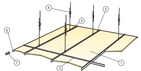
M46 Installation diagram (M46) for Ecophon Focus A XL
