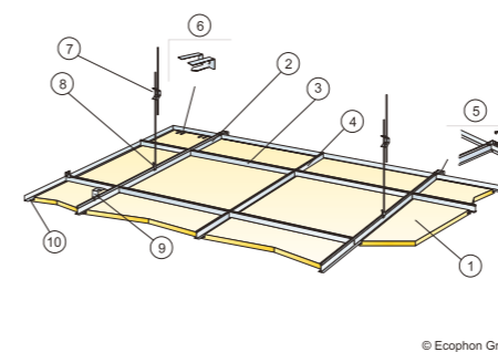
M203 Installation diagram (M203) for Ecophon Focus Dg 1200x1200 mm
