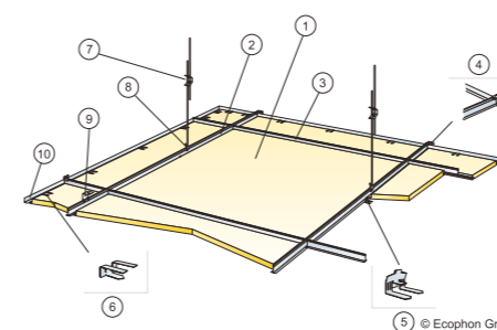
M203 Installation diagram (M203) for Ecophon Focus Dg 1200x1200 mm
