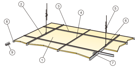
M01 DIN Installation diagram (M01 DIN) for Ecophon Focus A
