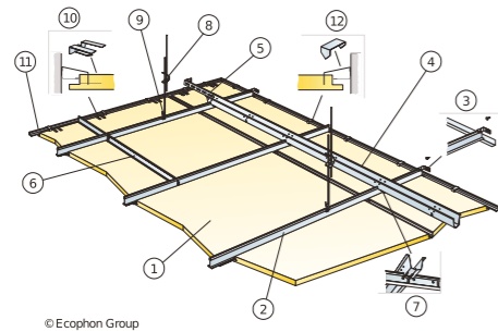
M206 Installation diagram (M206) for Ecophon Focus Ds 600x600, 1200x600 mm and Ecophon Focus Ds XL. Suspended installation
