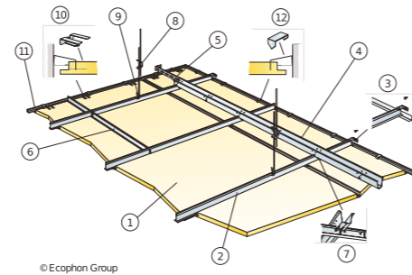
M206DIN Installation diagram (M206DIN) for Ecophon Focus Ds 625x625, 1250x625 mm. Suspended installation
