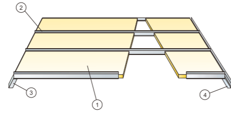
M16 Installation diagram (M16) for Ecophon Focus A XL in corridors
