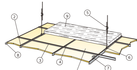
M399 Installation diagram (M399) for Ecophon Focus A
