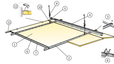
M207 Installation diagram (M207) for Ecophon Focus Ds 1200x1200 mm
