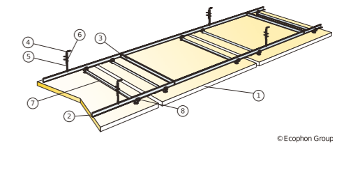
Installation diagram (M502) for Ecophon Solo Matrix in rows
