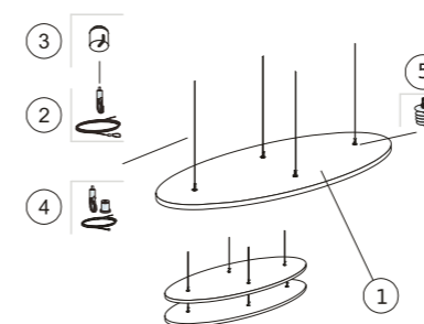
M428 Installation diagram (M428) for Ecophon Solo Ellipse
