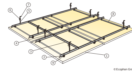
Installation diagram (M503) for Ecophon Solo Matrix in modules
