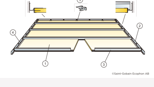
M238 Installation diagram (M238) for Ecophon Focus Ds XL in corridors
